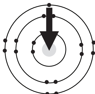
Chlorine
